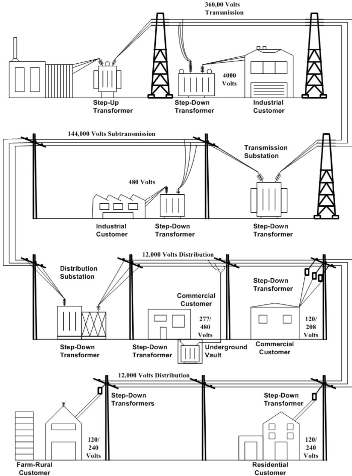
Electrical supply from generator to customer showing transformer applications and typical operating voltages.
