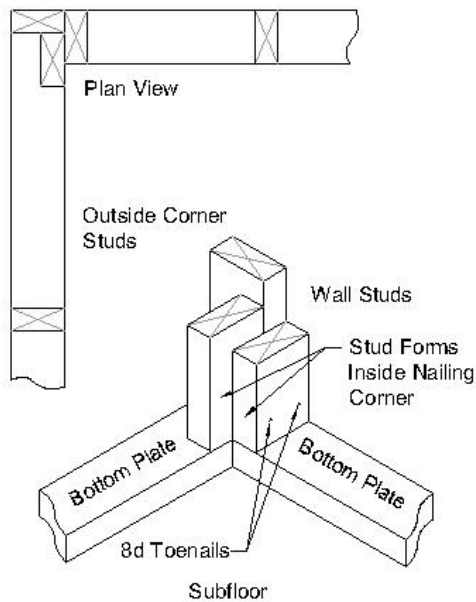
(A) Outside corner construction using only three studs.
