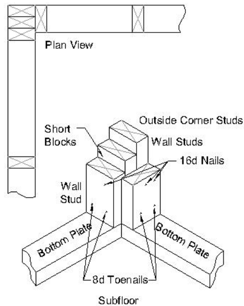
(B) Outside corner construction using two studs with short blocks between them at the center and ends. A third full length stud can be used instead of blocks.
