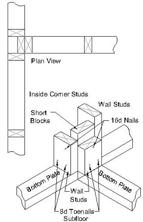
(C) Inside corner construction using a block laid flat. A full length stud can be used instead of a block.
